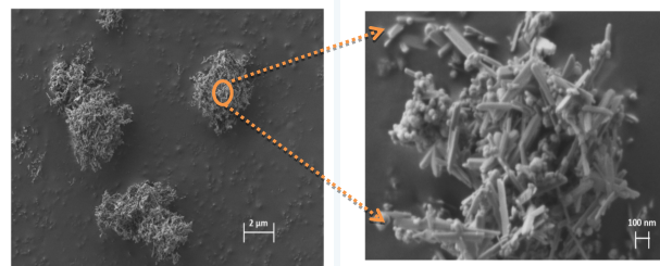
Figure 1: FE-SEM images of the ionic liquid-Fe 3 O 4 core @ chitosan magnetic nanoparticles.
