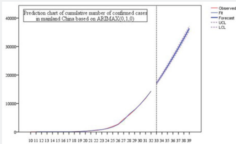
Figure 4: Prediction chart of cumulative number of confirmed cases in mainland China based on ARIMAX(0,1,0).
