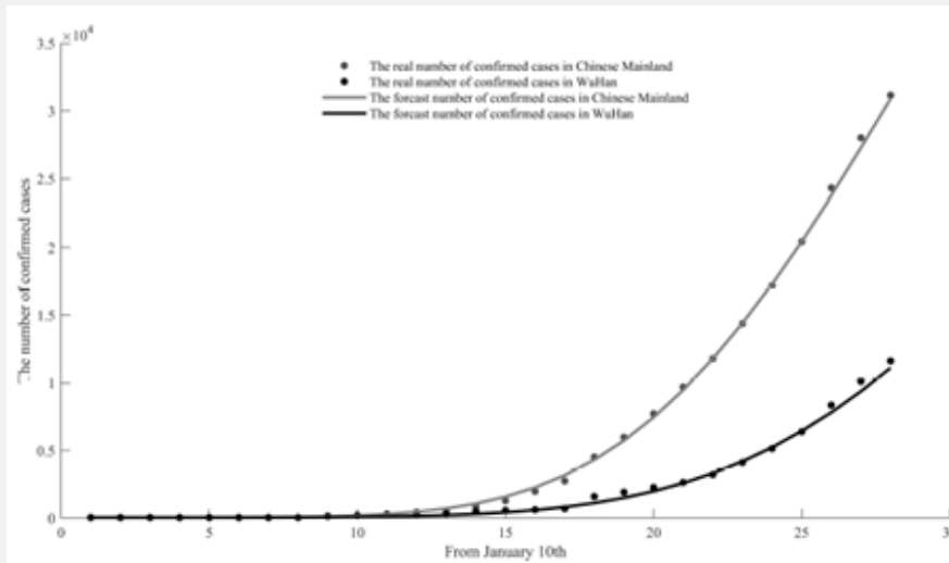
Figure 7: Matching effect chart of the real value and predicted value of the cumulative number of confirmed cases in China and Wuhan.
