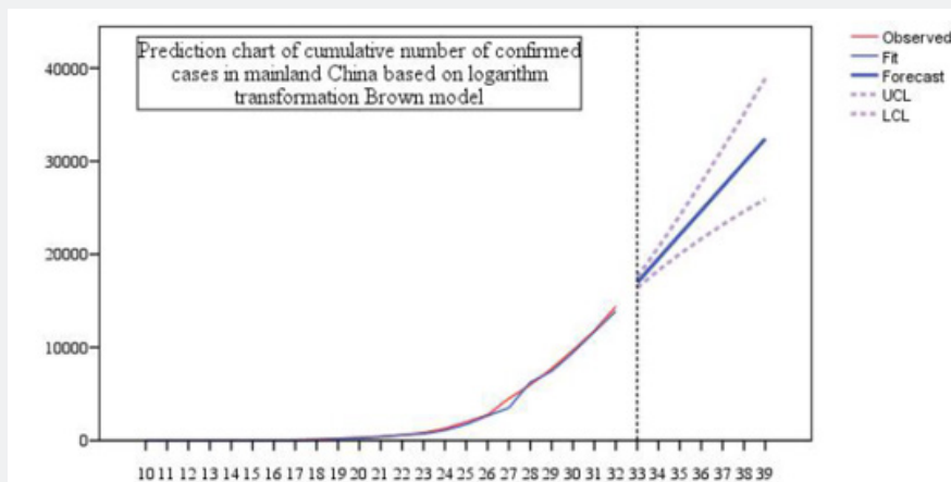
Figure 3: Prediction chart of cumulative number of confirmed cases in mainland China based on logarithm transformation Brown model.
