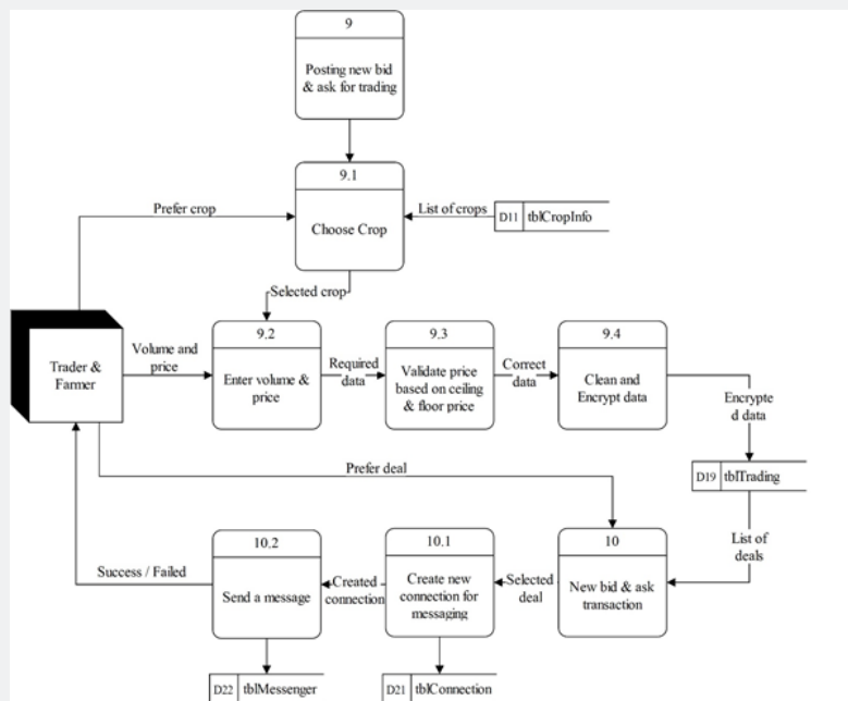
Figure 7: Level 1 Data Flow Diagram of Trading.
