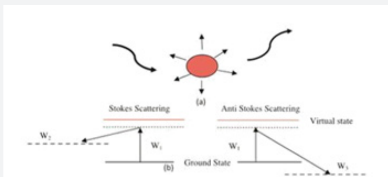
Figure 2: Basic principle of Raman spectroscopy: (a) a small portion of photons incident on a target molecule scatters with a shift in photon energy due to molecular vibration, (b) energy diagram representing the process of scattering.
