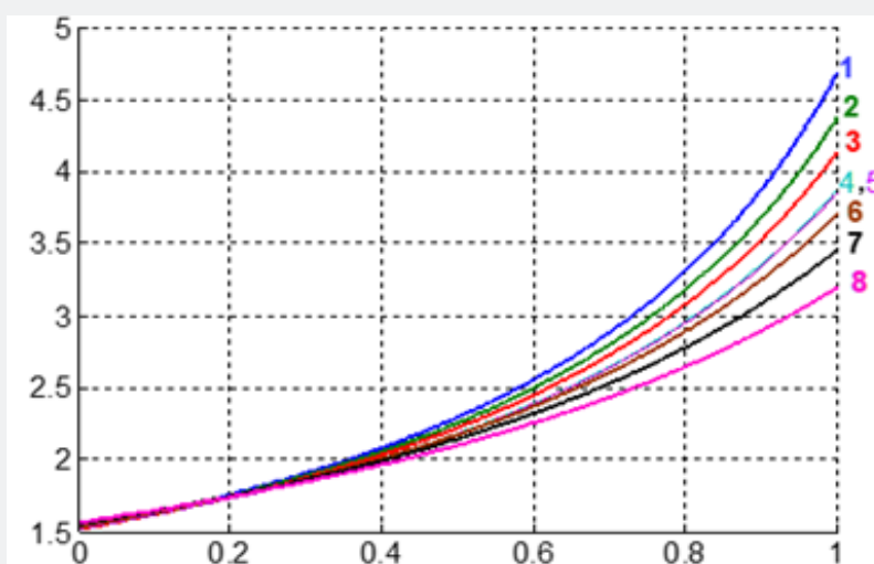
Figure 5: Dependence of stress index S = \mu/(1-\theta D) of different LS on probability D of achieving maximal population size. Life systems names and parameters values \mu and \theta are given in Table 2
