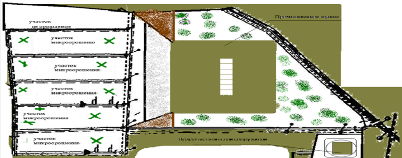
Figure 1: Scheme of the irrigation sprinkling station on the experimental part of the Tertersky RWCN in the Garabagh land in the period 2006-2010 with the use of the Idad and MDR sprinklers.
