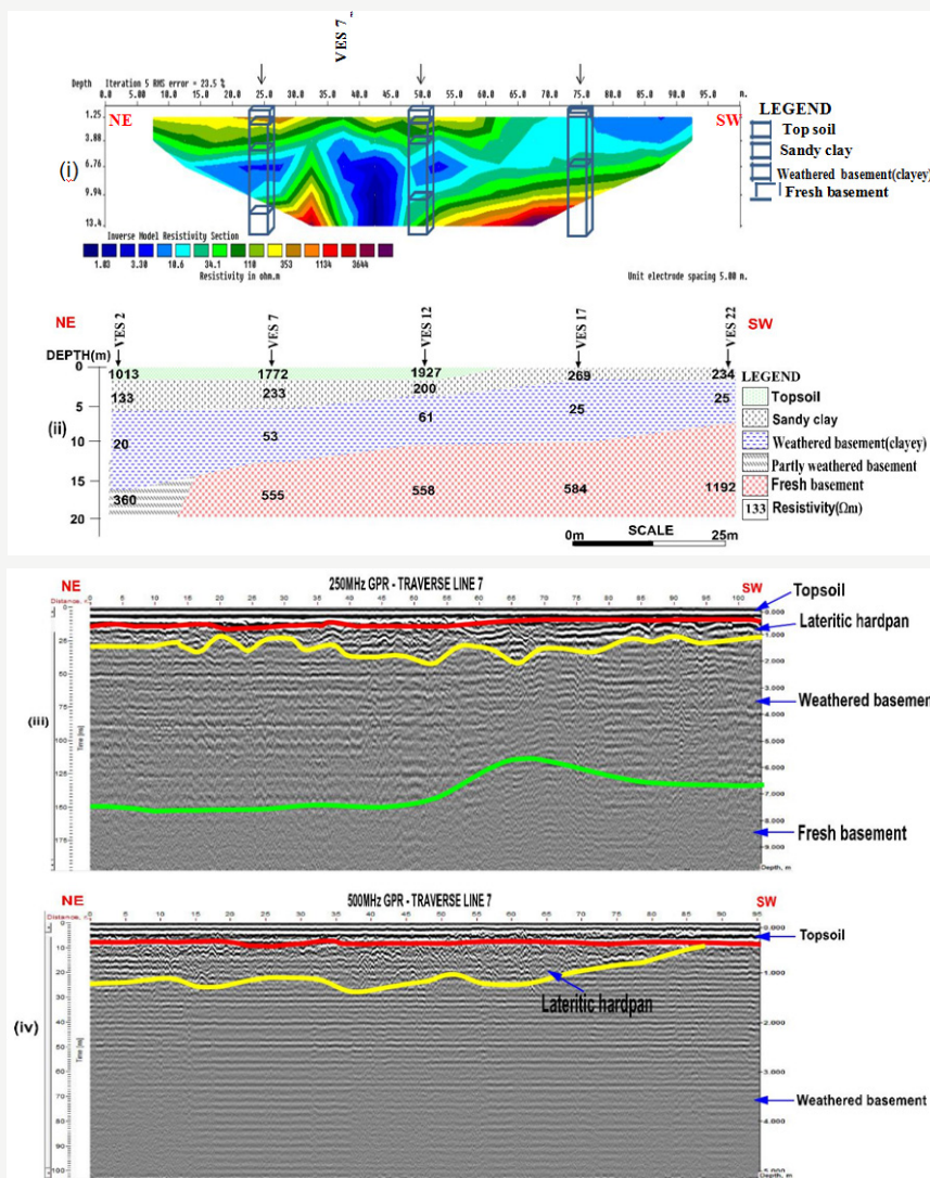
Figure 10: Correlation of (i) Inverted resistivity section (ii) Geoelectric section (iii) Radar section for 250 MHz antenna and (iv) Radar section for 500 MHz antenna beneath Traverse 7.
