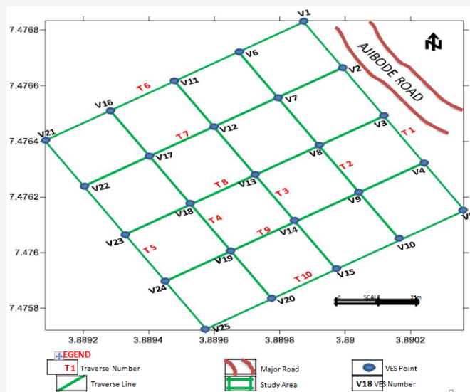
Figure 3: Field Layout of the study area.
