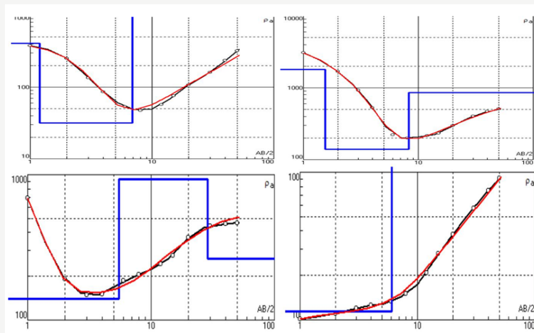
Figure 4: Representative curve types from the study area.
