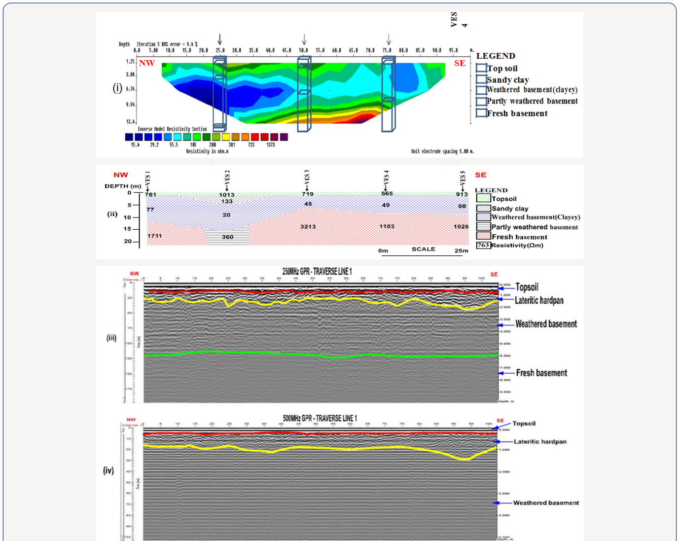
Figure 9: Correlation of (i) Inverted resistivity section (ii) Goelectric section (iii) Radar section for 250 MHz antenna and (iv) Radar section for 500 MHz antenna beneath Traverse 1.
