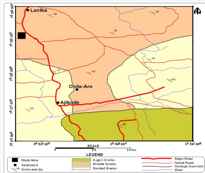
Figure 2: Geological map of Ajibode (Modified after Oyediran and Adeyemi, 2011).
